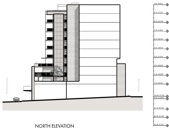
NORTH ELEVATION
