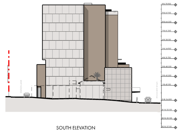
SOUTH ELEVATION
