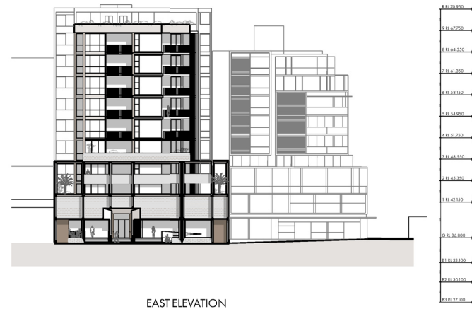
EAST ELEVATION
